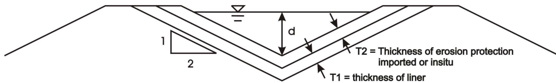
Figure 3 – Design canal cross sections utilised
